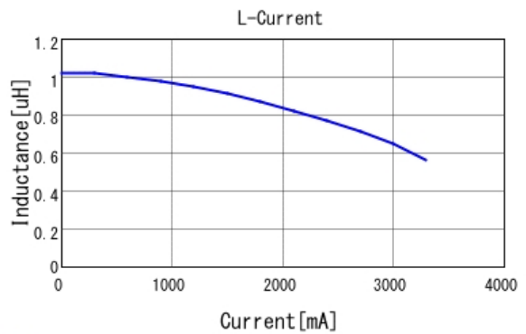
■ 1285AS-H-1R0M L-Current 20degC
