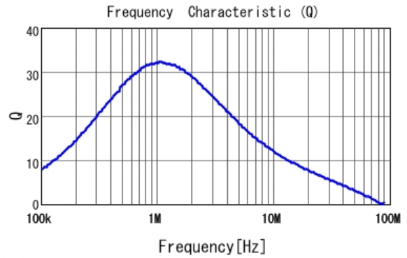
■ 1285AS-H-1R0M Q
