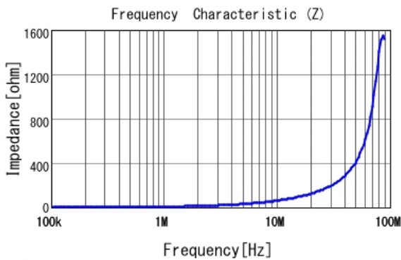
■ 1285AS-H-1R0M |Z|
