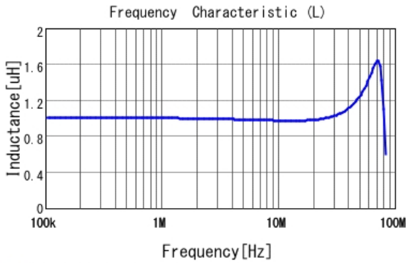
■ 1285AS-H-1R0M L
